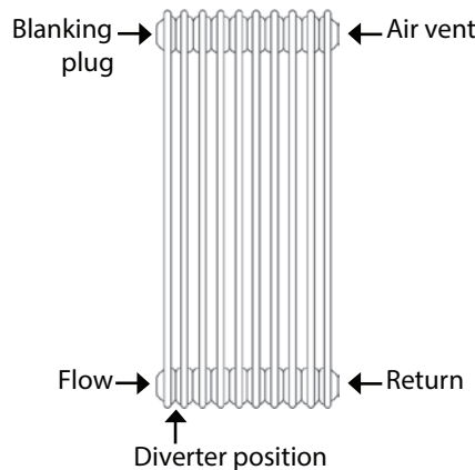
Drawing 2 - Steel Multi Column Orientation
